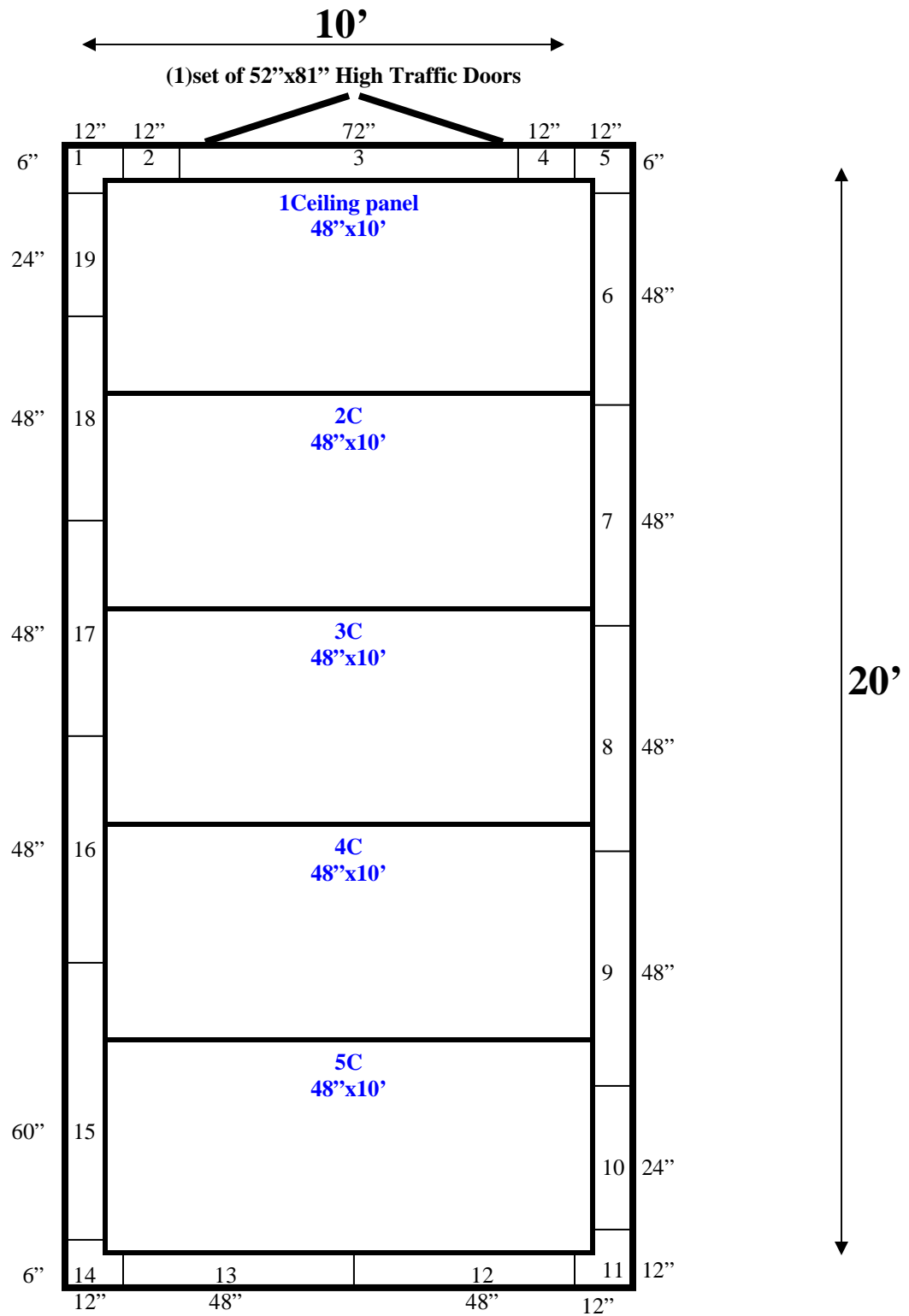
10' x 20' x 8'4" H Walk-In Cooler or Freezer Wall & Ceiling Panels Diagram
