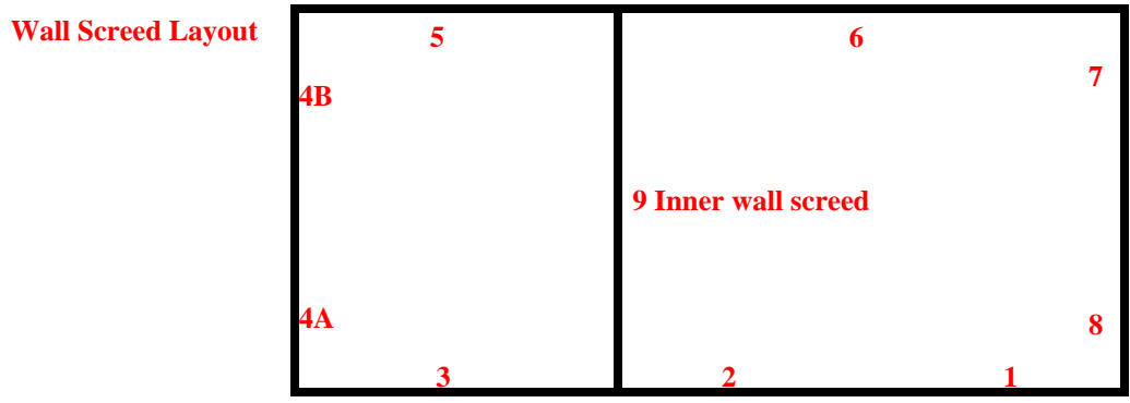
7'8" x 19'4" x 8'6"/10'6" H Walk-In Combination Cooler / Freezer Wall, Ceiling Panels, & Floor Screed Diagram
