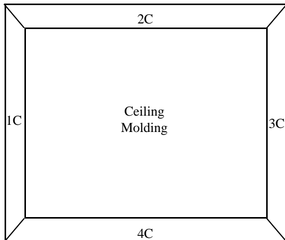
7'9" x 8'5" x 8'4" H New Walk-In Cooler Panel Layout Diagrams
