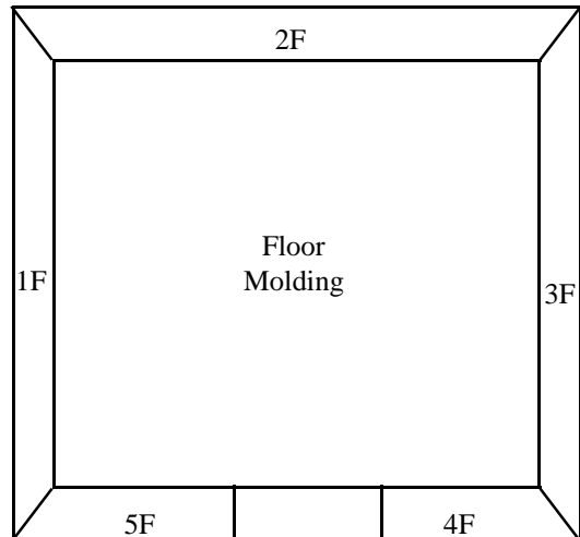
8'5" x 11'7" x 8'4" H New Walk-In Cooler Panel Layout Diagrams
