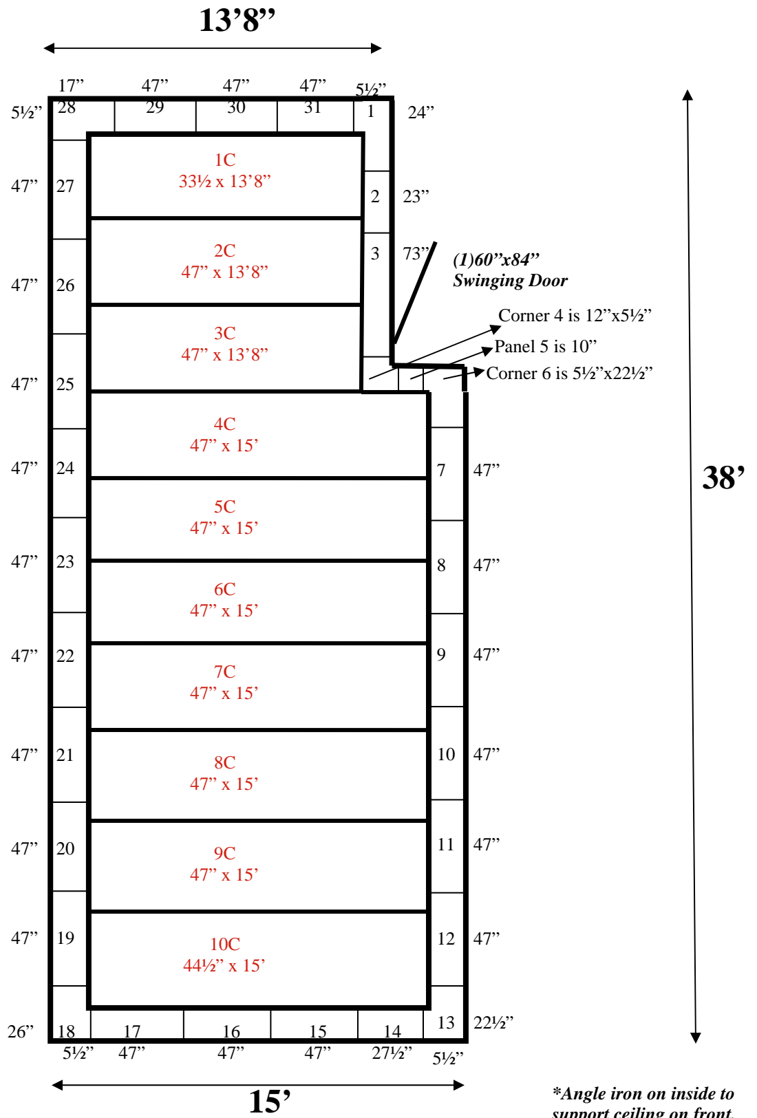
15' x 38' x 9' H Walk-In Cooler or Freezer Wall and Ceiling Panels Diagram
