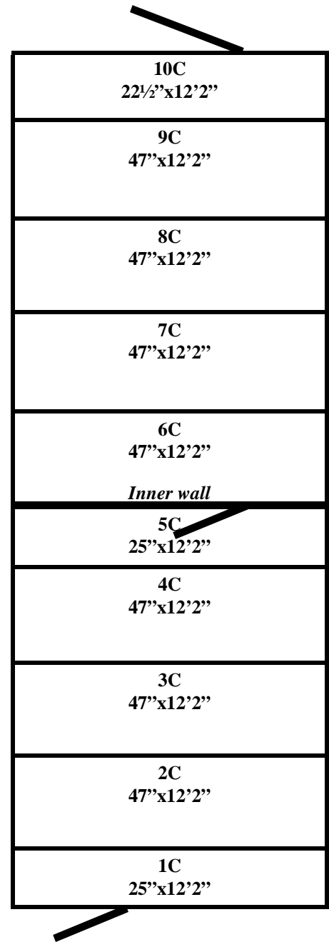
Ceiling Panels Diagram
