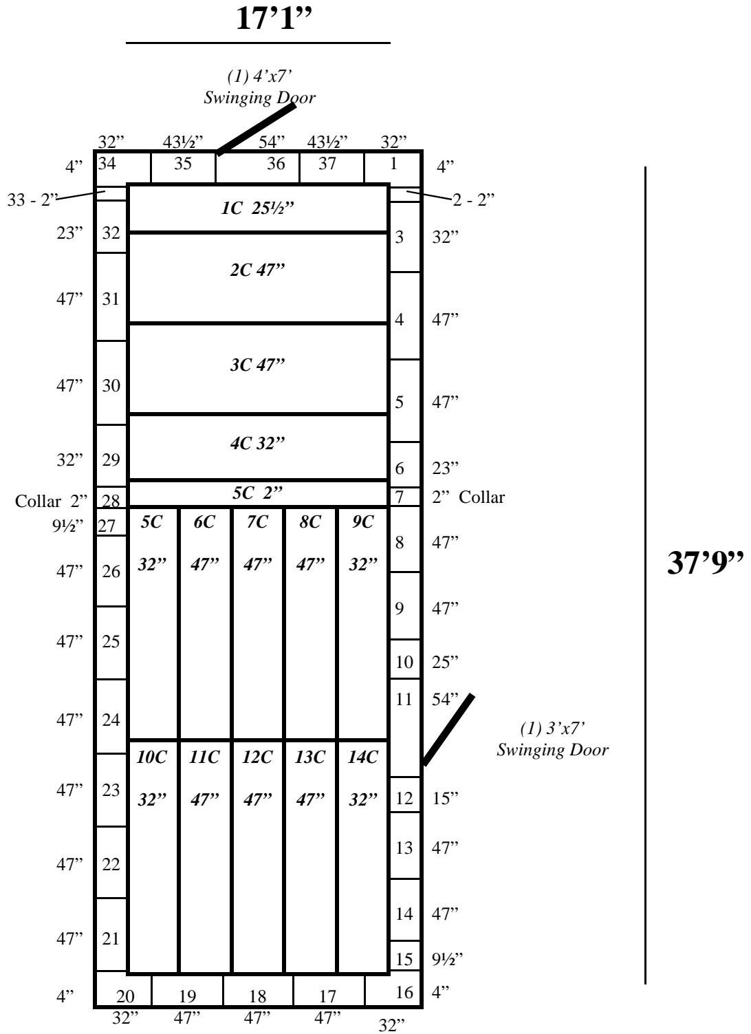
17'1" x 37'9" x 10'3" H Red Orange Walk-In Cooler or Freezer Wall and Ceiling Panels Diagram
