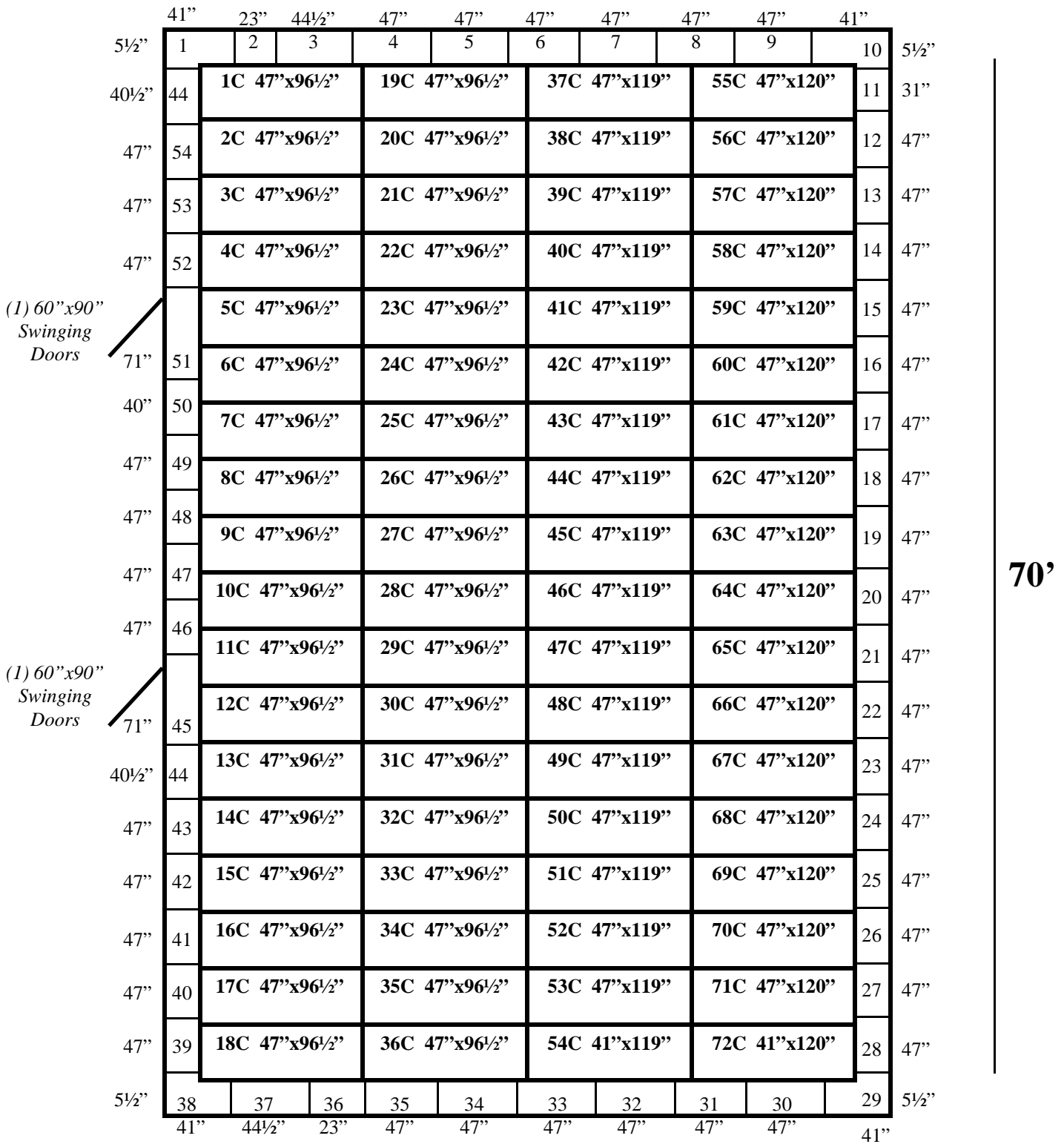
36' x 70' x 9'6" H Green Walk-In Freezer with Floor Wall and Ceiling Panels Diagram
