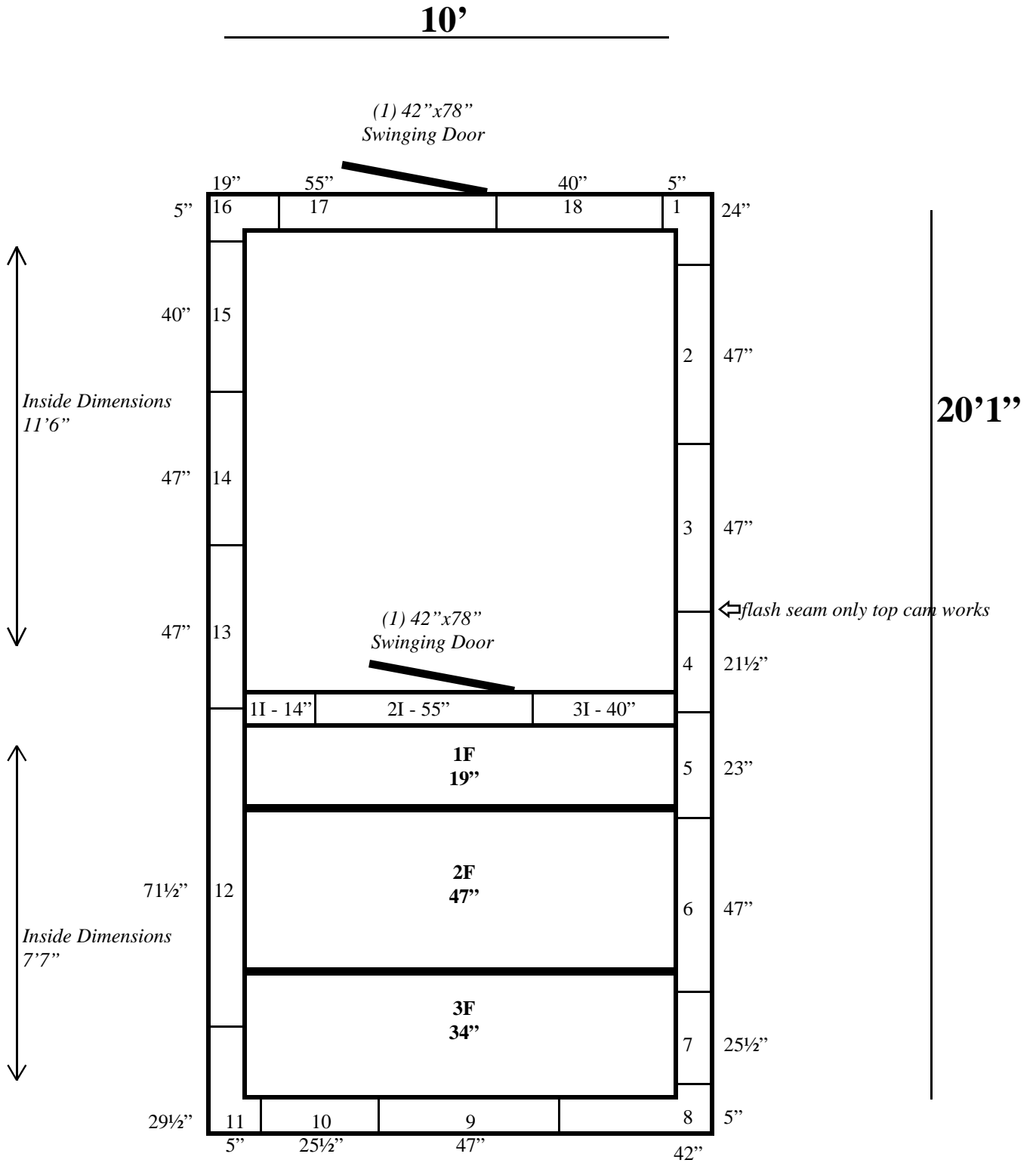
10' x 20'1" x 9'11" H Yellow Walk-In Combination Cooler / Freezer Wall & Floor Panels Diagram
